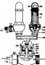
Figs. 2460-2461. Duplex Pump Governor, S D-4.
